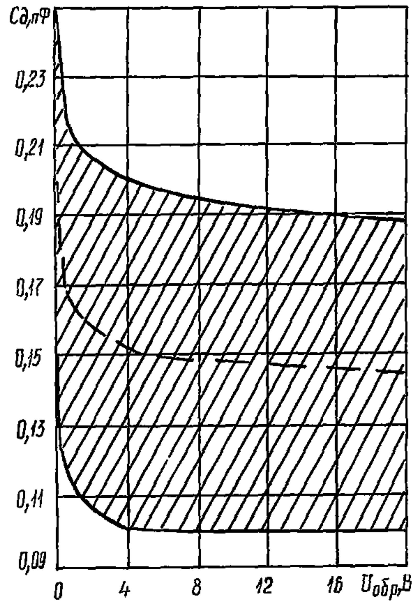
2A551В-3, 2A551Г-3
