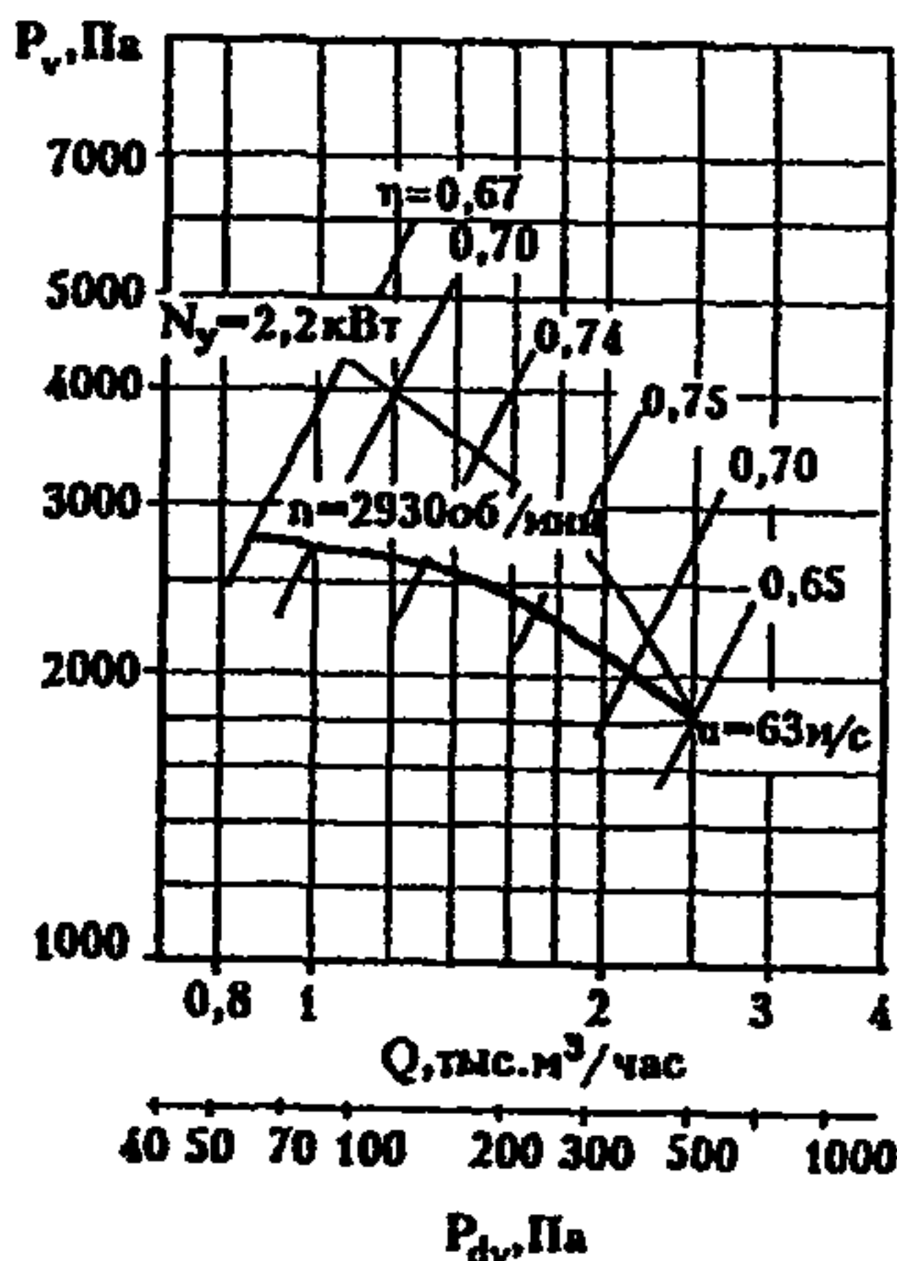
В.Ц5-35-8,5.01
