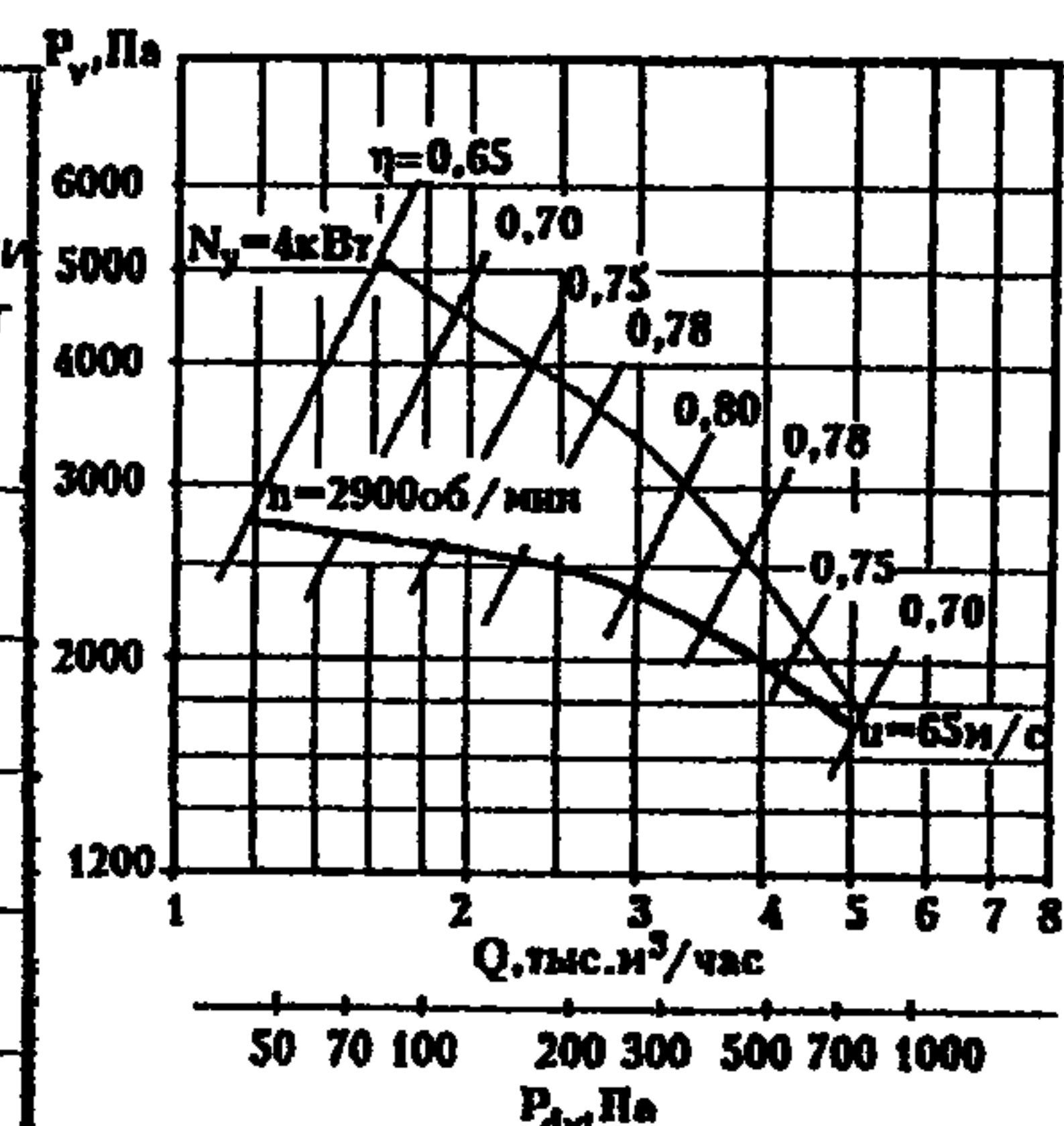
В.Ц5-45-8,5.01
