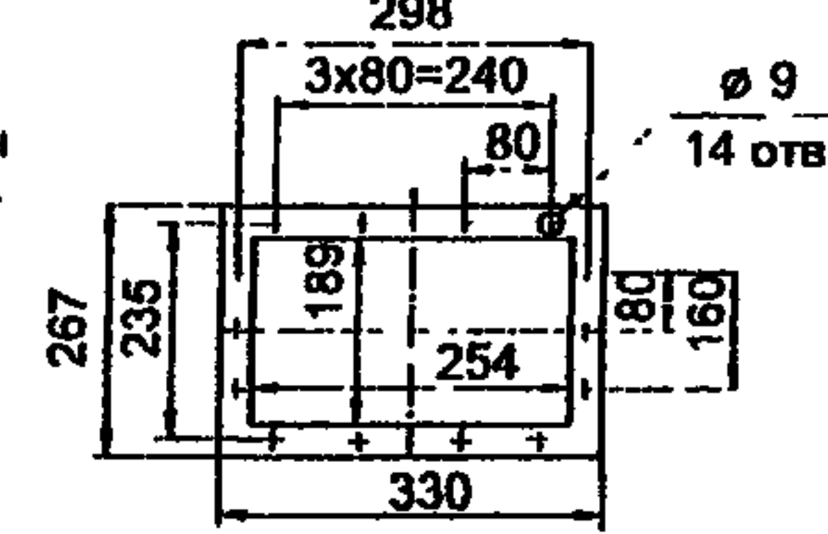
ВР132-30-10-02
