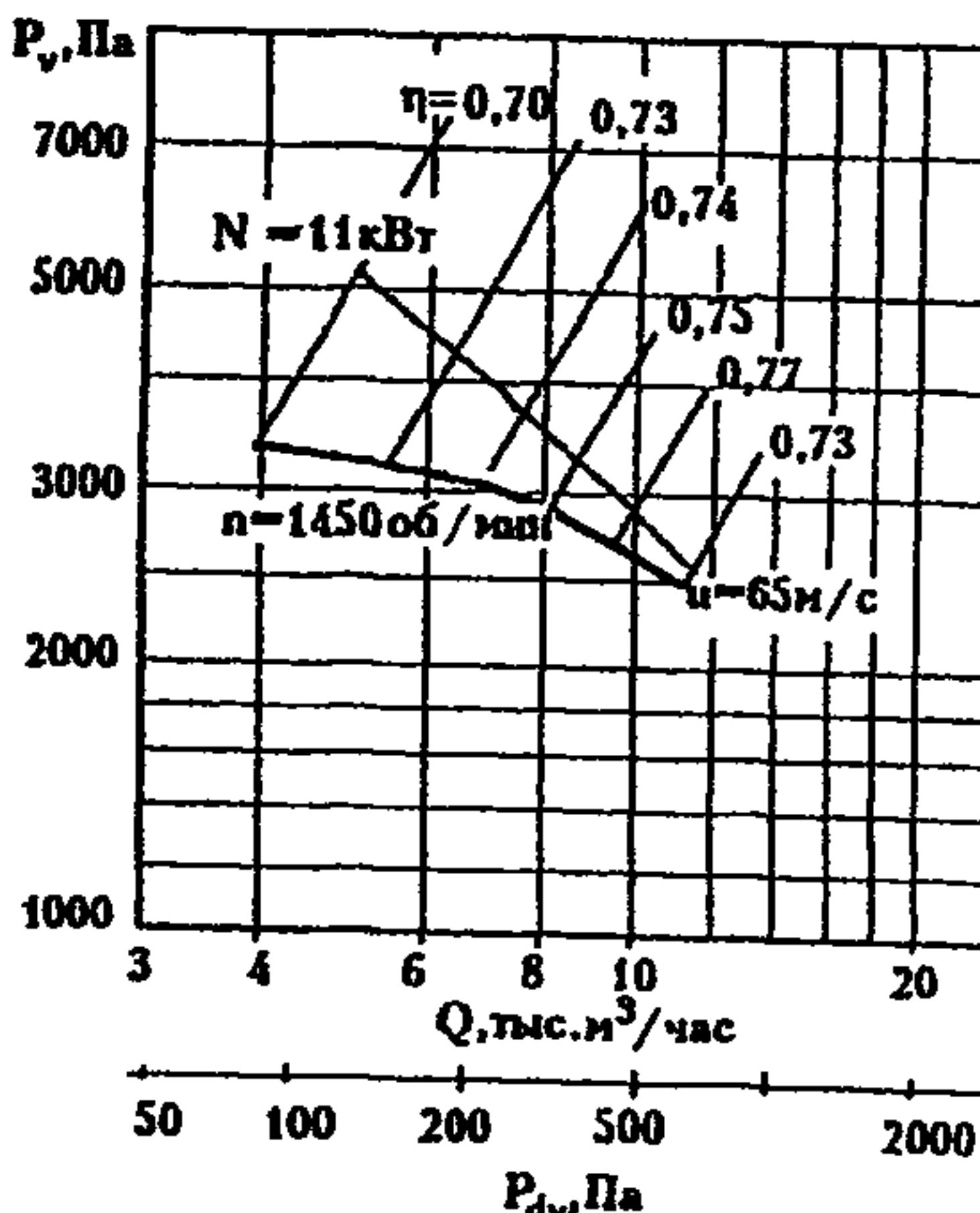
В.Ц5-35-8,5.01
