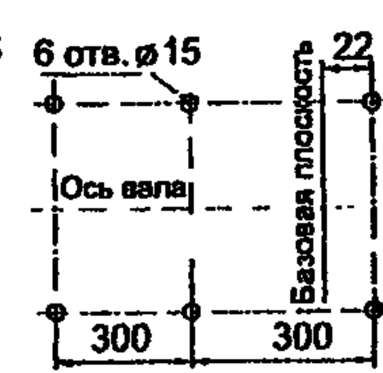
ВР132-30-10-02
