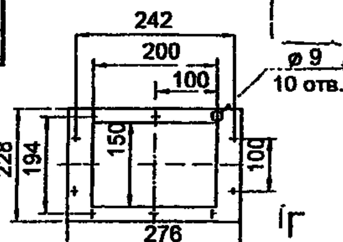
ВР132-30-10-02
