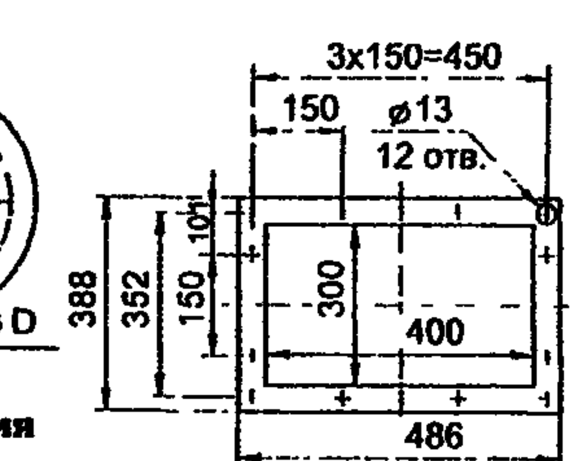
ВР132-30-10-02
