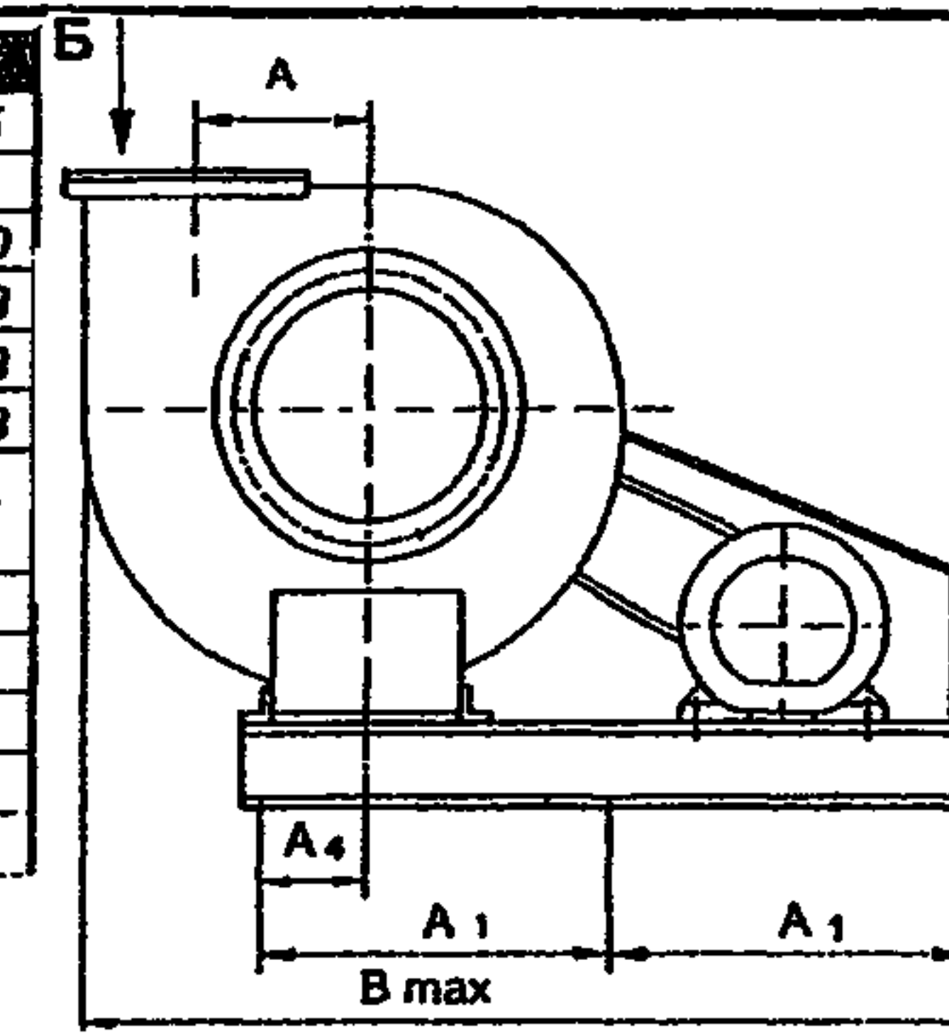
ВР132-30-10-01
