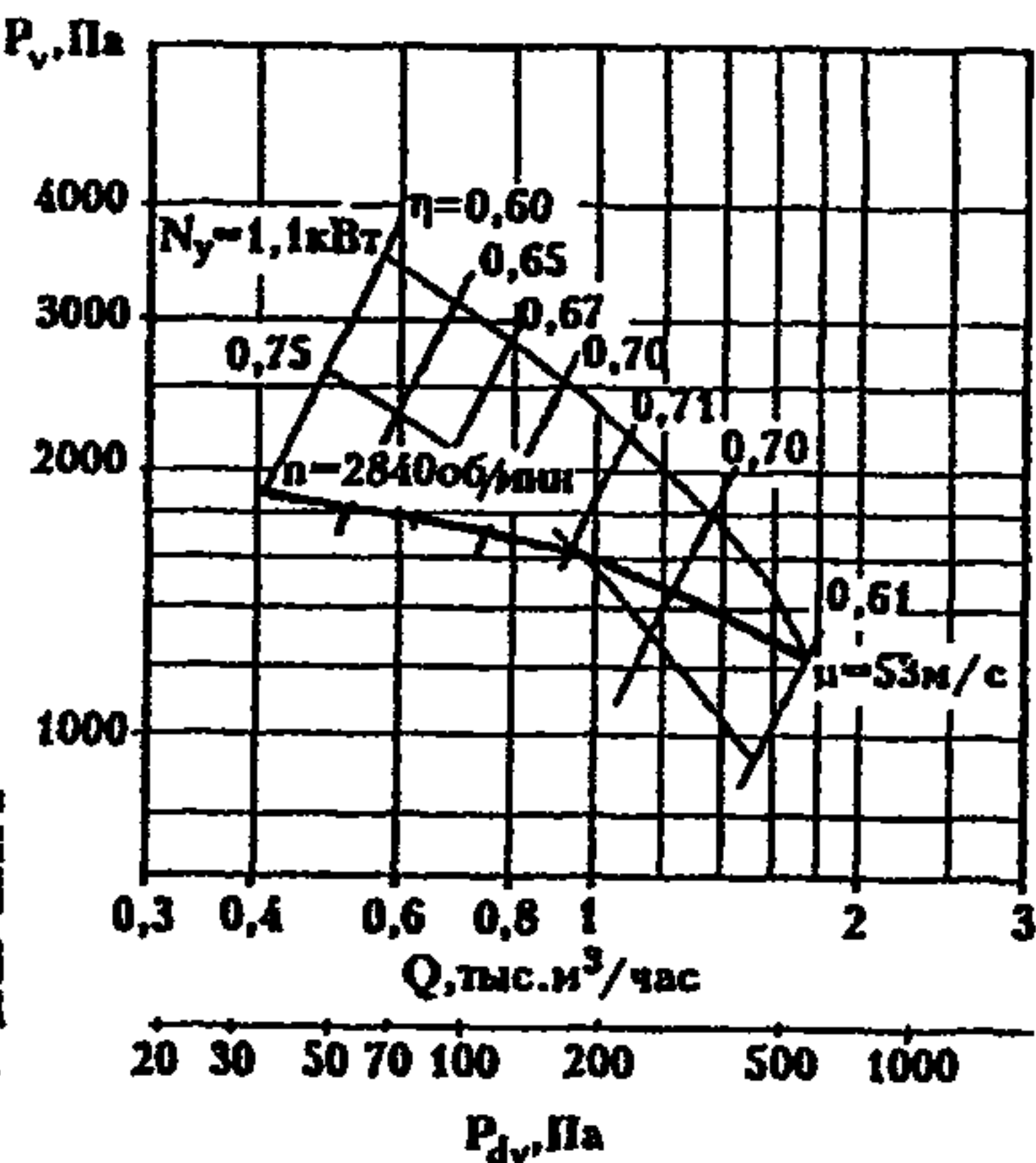
В.Ц5-35-3,55.01
