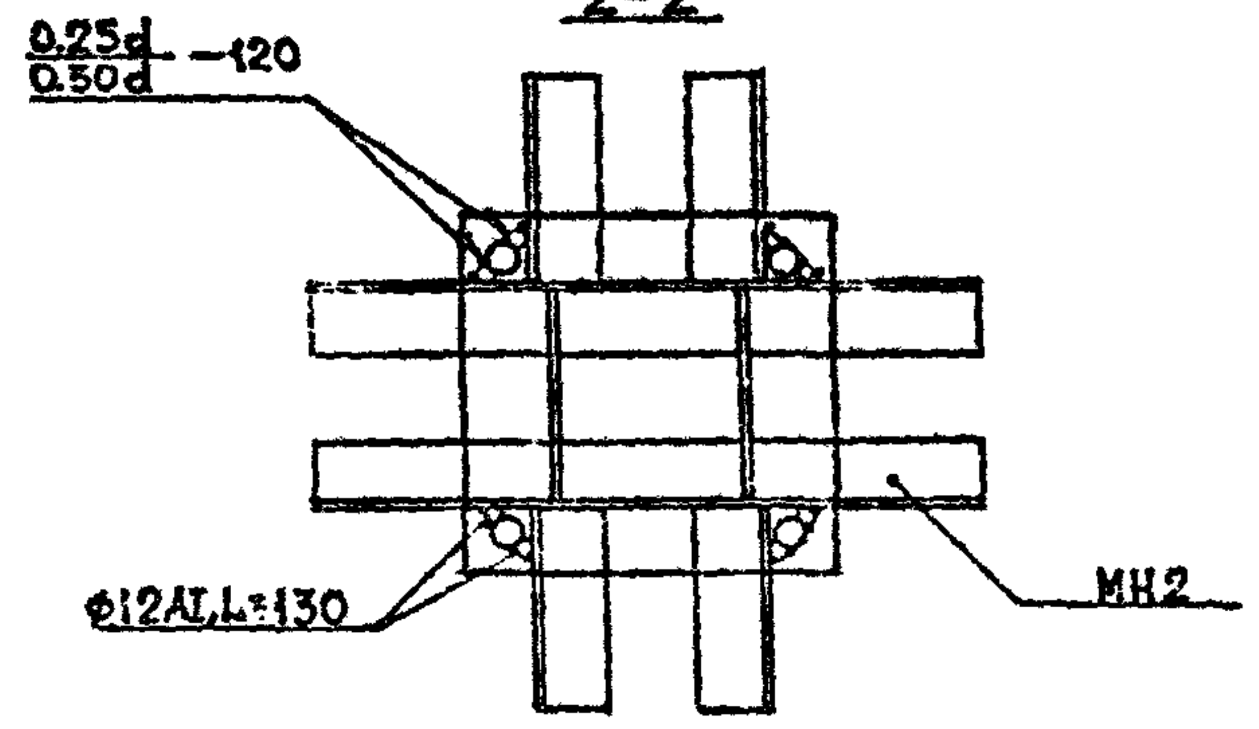
2-2
