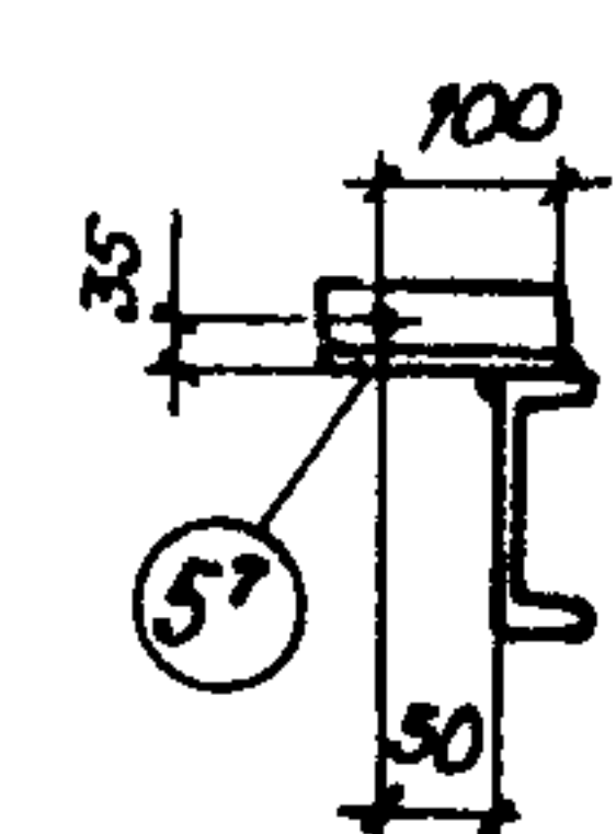
21-21
