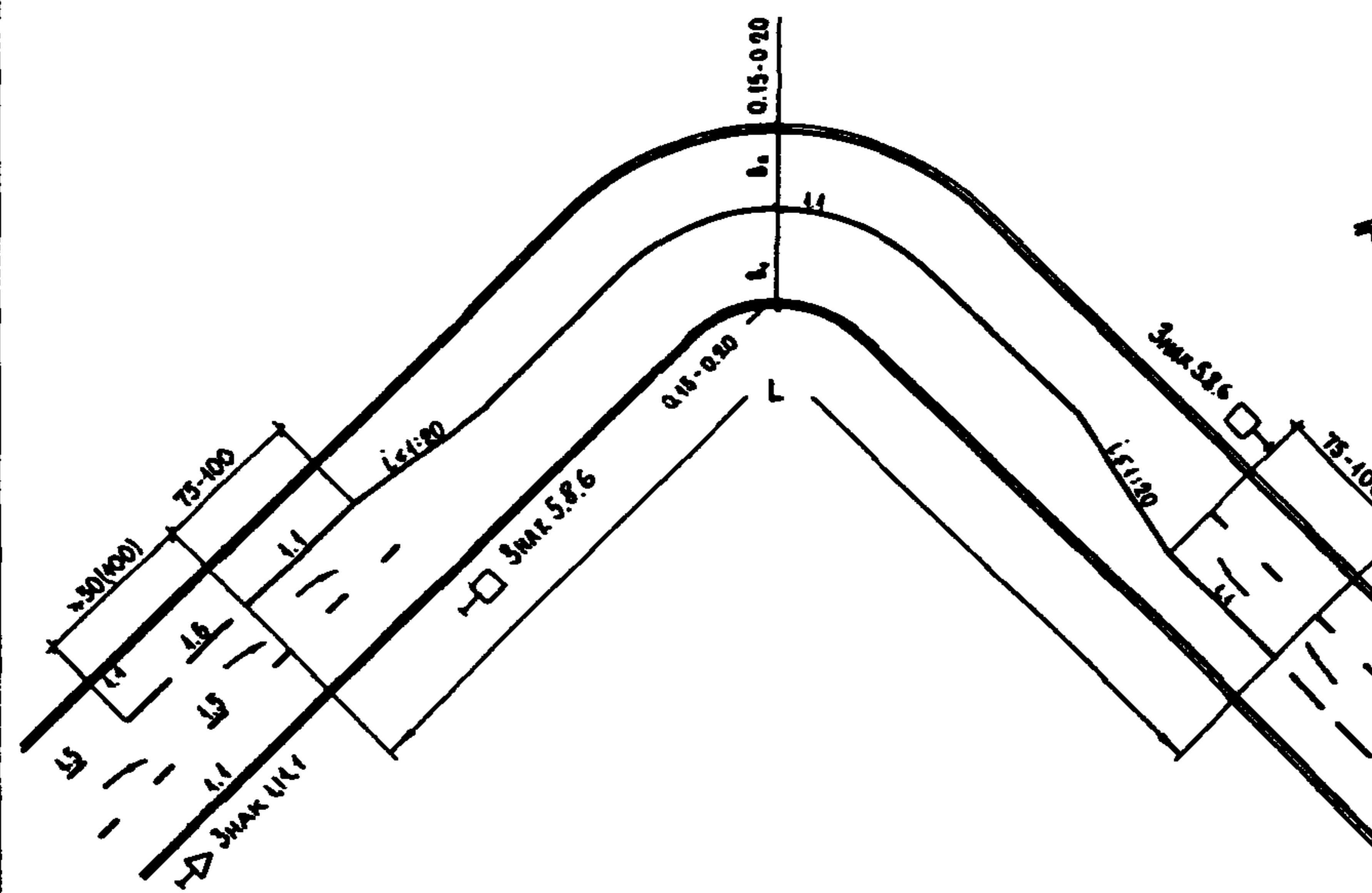
Б. При P = 1,0 - 5,0
